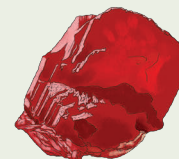
Fig. 9.5: Cinnabar
