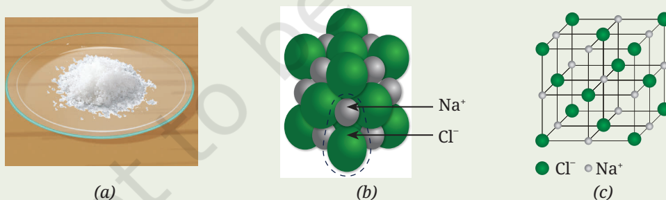
Fig. 9.14: Sodium chloride: (a) crystals, (b) crystal structure, and (c) crystal lattice
